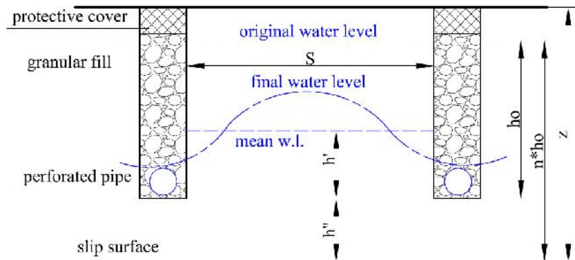
(Fig.1) Effect of trenches in the underground water table.
