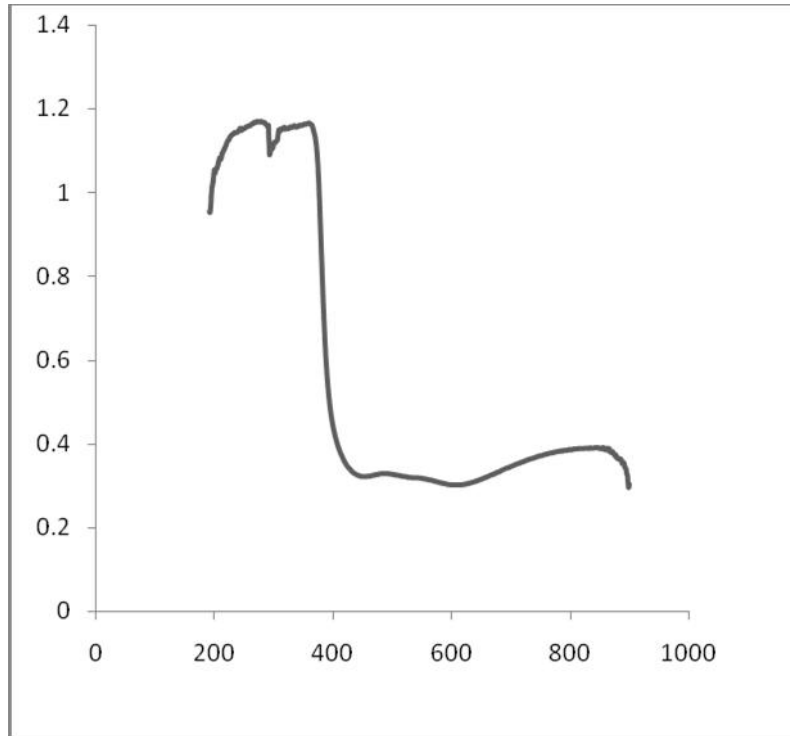
Figure 1: UV-DRS of ZnO/Al 2 O 3 (400) Base(482)
